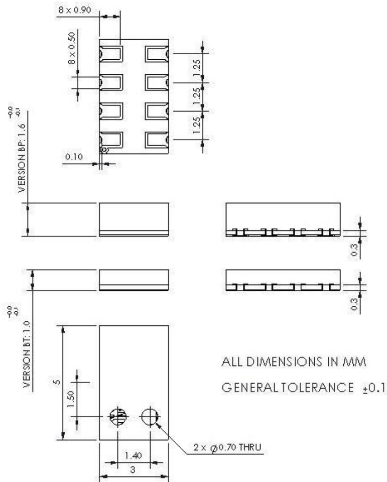
Figure 18: MS5607 package outline
