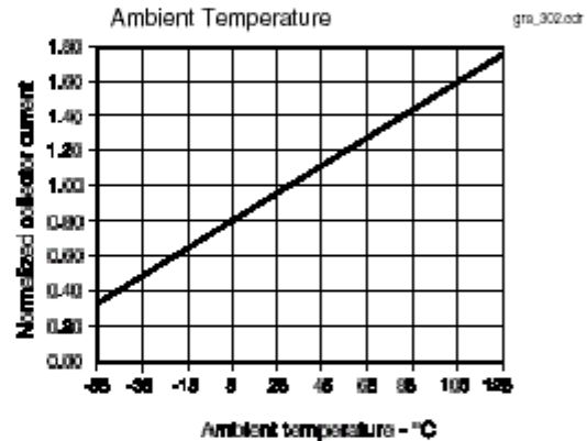
Fig. 8 Collector Current vs Ambient Temperature
