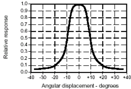
Fig. 2 Responsivity vs Angular Displacement (SD5443)
