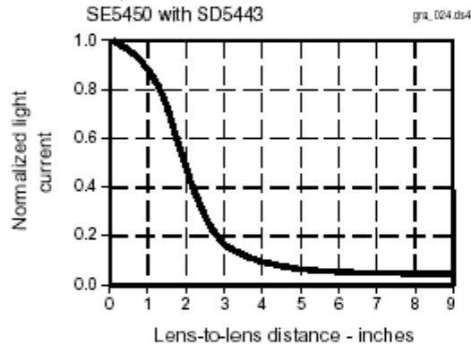
Fig. 7 Coupling Characteristics SE5450 with SD5443
