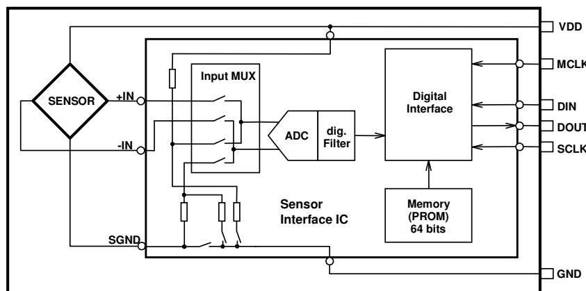
Fig. 1: Block Diagram MS5536-60C
